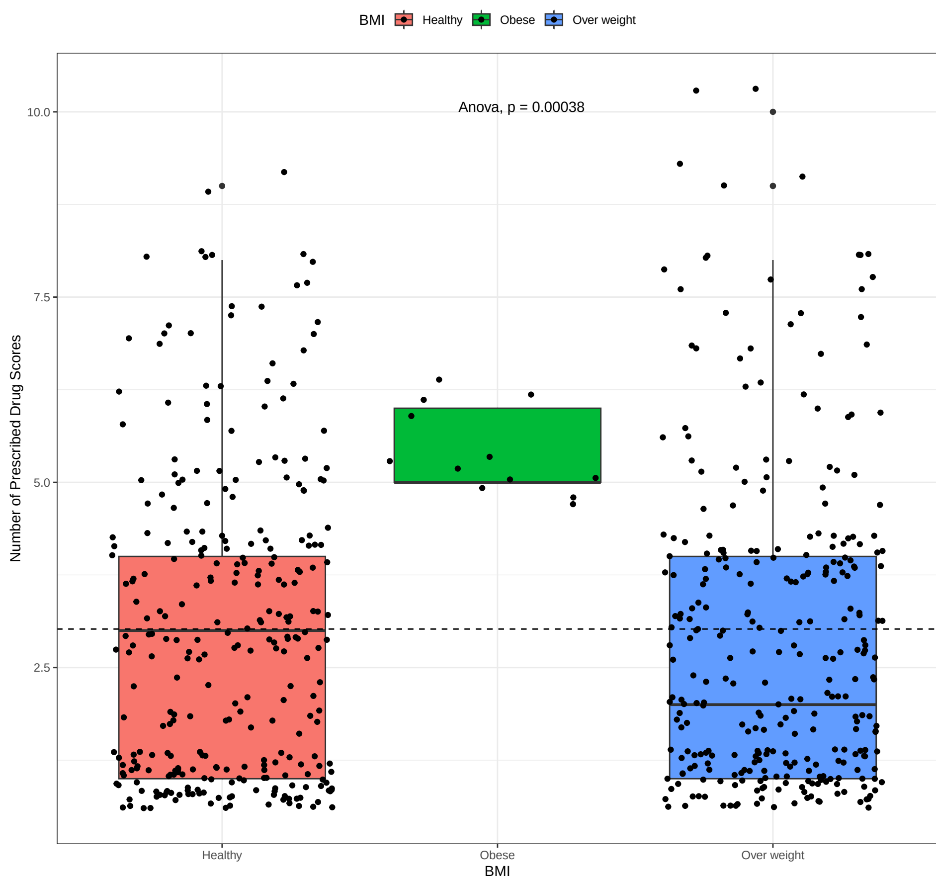
Distribution of Number of Prescribed Drug Scores among BMIs
